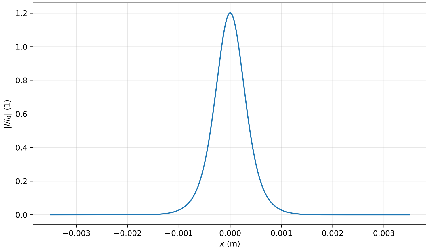
Intensity profile I(x, y = 0, z = 1.433m)/I_0 , P_{in}=0.7P_{cr} , artificial time
